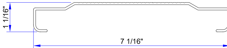
1 x 7 CI-RISER ( ALCOA # ????? )
