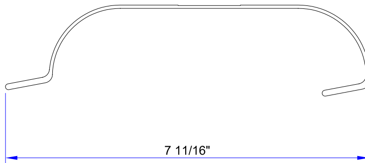
CONTOURED SEAT BACK ( ALCOA # 11530 )
