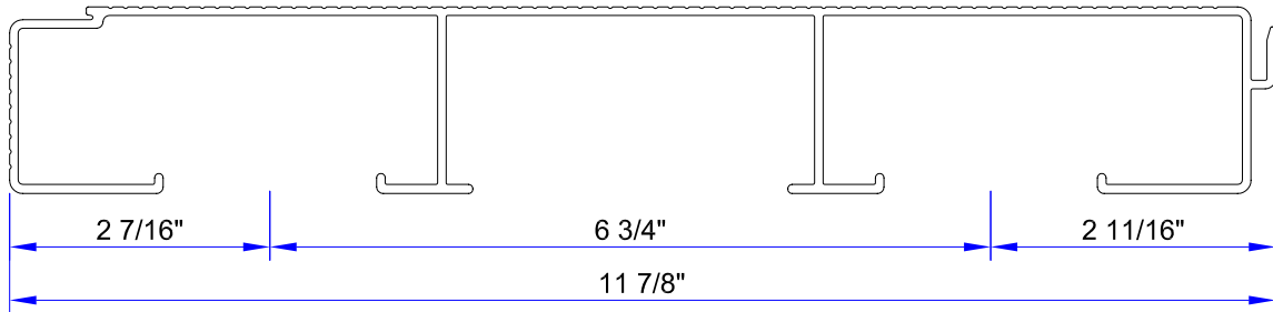
2 x 12 STEP BOARD ( ALCOA # 69972 )
