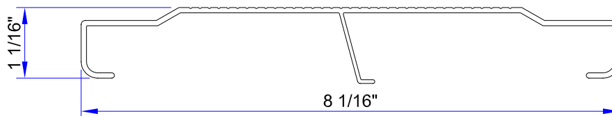
1 x 8 CI-RISER ( ALCOA # 69850 )
