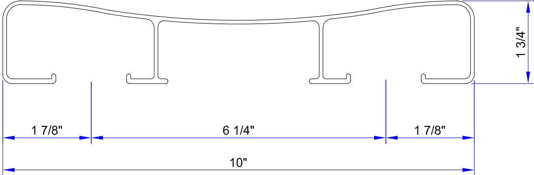
10" CONTOURED SEAT( ALCOA # 68754 )
