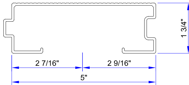
2 x 5 IL- DECK ( ALCOA # 69965 )
