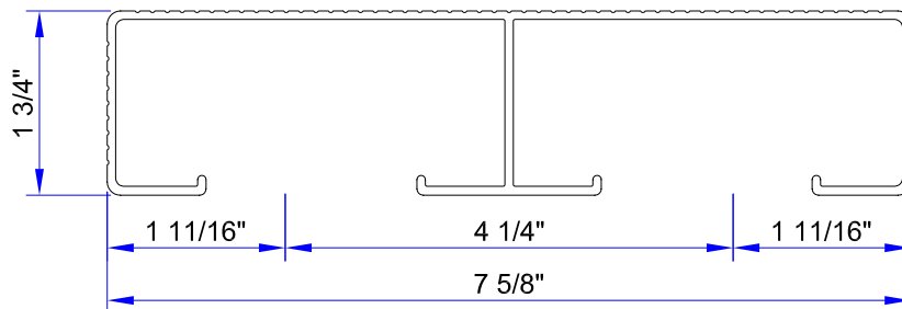
2 x 8 SC-DECK ( ALCOA # 69962 )
