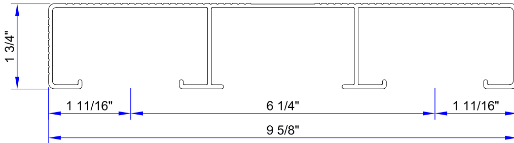
2 x 10 SC-DECK ( ALCOA # 69959 )
