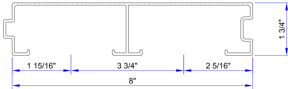
2 x 8 IL- DECK ( ALCOA # 69803 )
