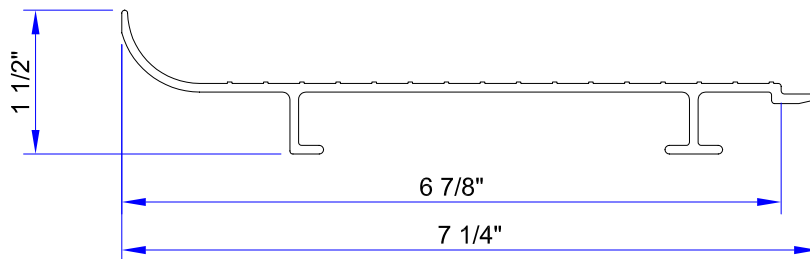
1 1/2 x 6 1/2 IL-RISER ( ALCOA # 69637 )
