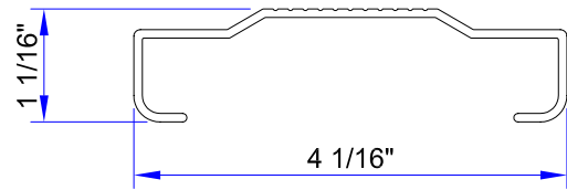
1 x 4 CI-RISER ( ALCOA # 69973 )
