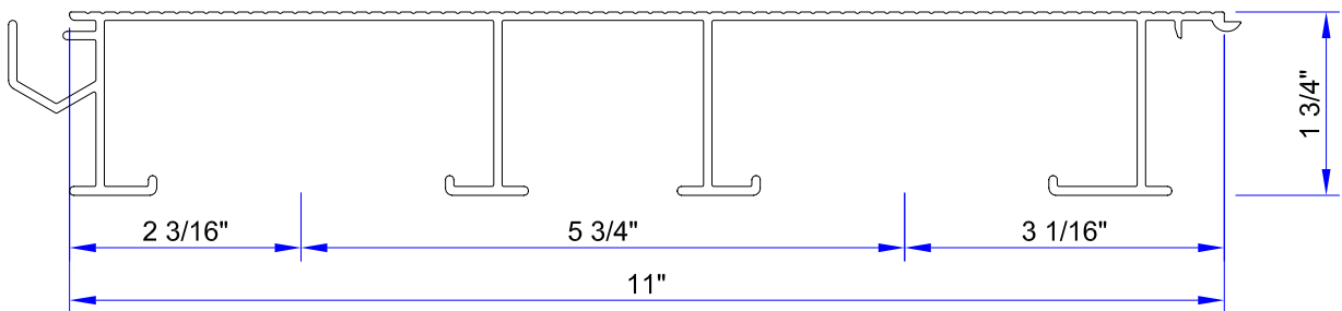
2 x 11 GI-DECK ( ALCOA # 69946 )
