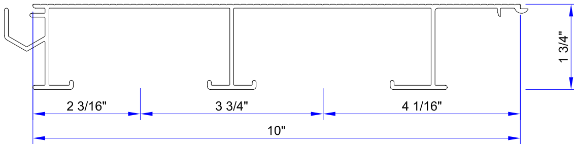
2 x 10 GI-DECK ( ALCOA # 69970 )
