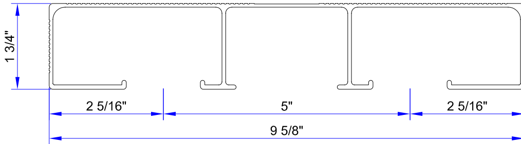
2 x 10 ( ALCOA # 60772 )
