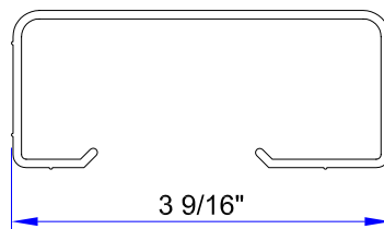
3 9/16" INSERT ( ALCOA # 65520 ) FOR 2 x 8 ( # 65482 )
