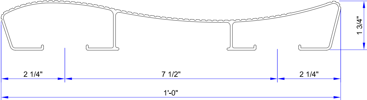
12" CONTOURED SEAT( ALCOA # 11965 )
