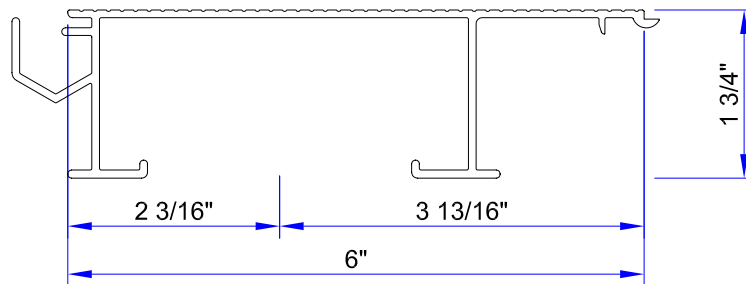
2 x 6 GI-DECK ( ALCOA # 69969 )
