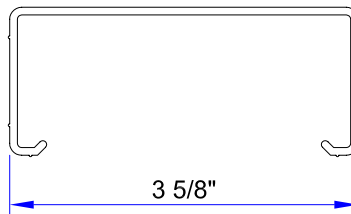
3 5/8" INSERT ( ALCOA # 69801 ) FOR ALL FOOT BOARDS IN THE CI, WD, GI, SERIES
