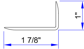
L-SHAPE END CAP ( ALCOA # 69664 )
