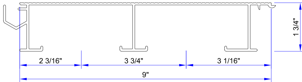
2 x 9 IL-DECK ( ALCOA # 69945 )
