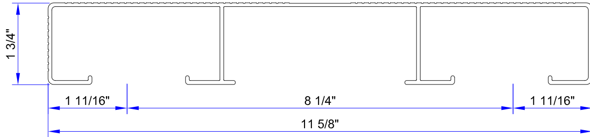
2 x 12 SC-DECK ( ALCOA # 69963 )
