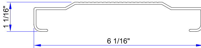
1 x 6 CI-RISER ( ALCOA # 69974 )
