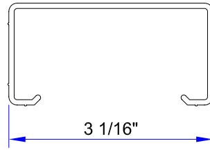
3 1/16" INSERT ( ALCOA # 69966 ) FOR 2 x 8, 2 x 10, 2 x 12 ( # 69962, 69959, 69963 )
