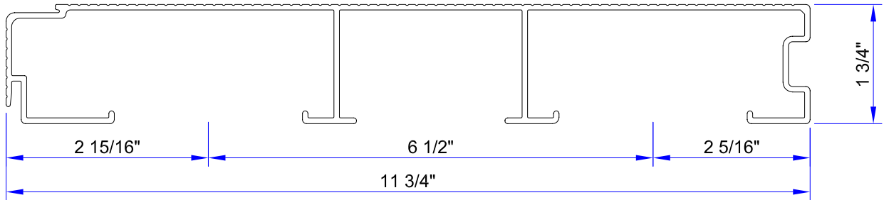
2 x 12 IL-NOSE ( ALCOA # 69961 )
