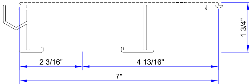
2 x 7 GI-DECK ( ALCOA # 69944 )
