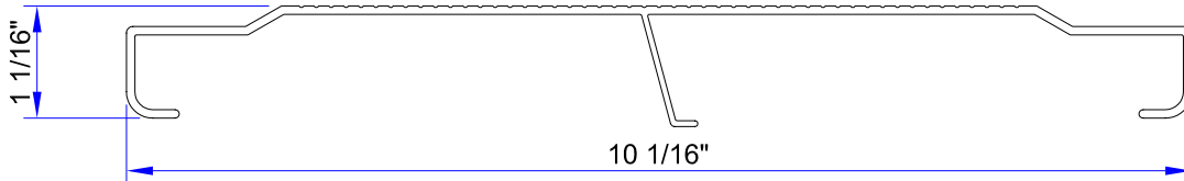
1 x 10 CI-RISER ( ALCOA # 69988 )
