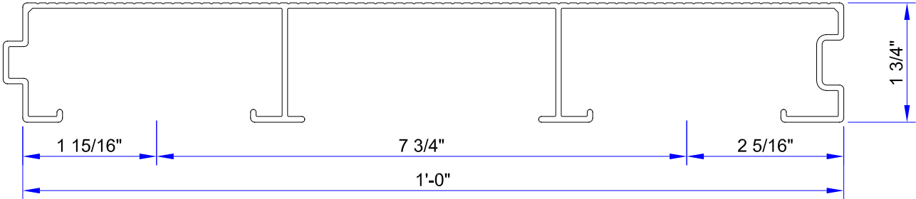
2 x 12 IL-DECK ( ALCOA # 69960 )
