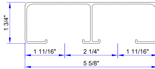
2 x 6 ( ALCOA # 12214 )
