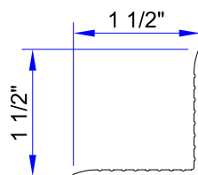
1 1/2" CLOSURE ( ALCOA # 66782 )
