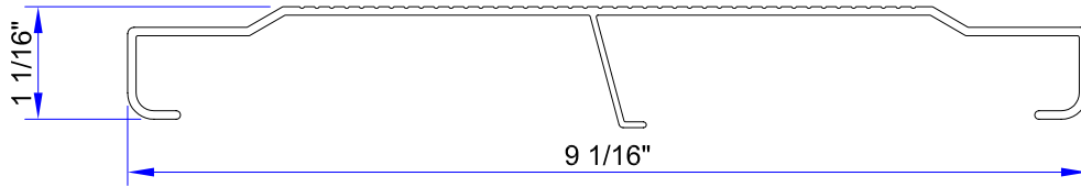
1 x 9 CI-RISER ( ALCOA # 69987 )
