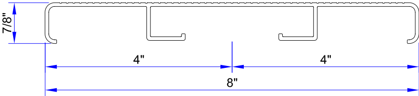
1 x 8 SC-RISER ( ALCOA # 70001 )
