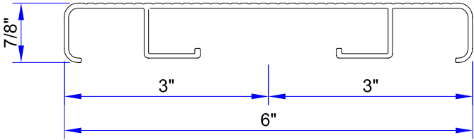
1 x 6 SC-RISER ( ALCOA # 70003 )
