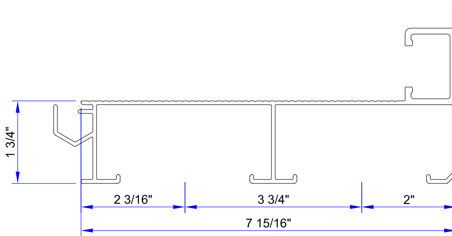
2 x 7 GI-HEEL ( ALCOA # 69943 )
