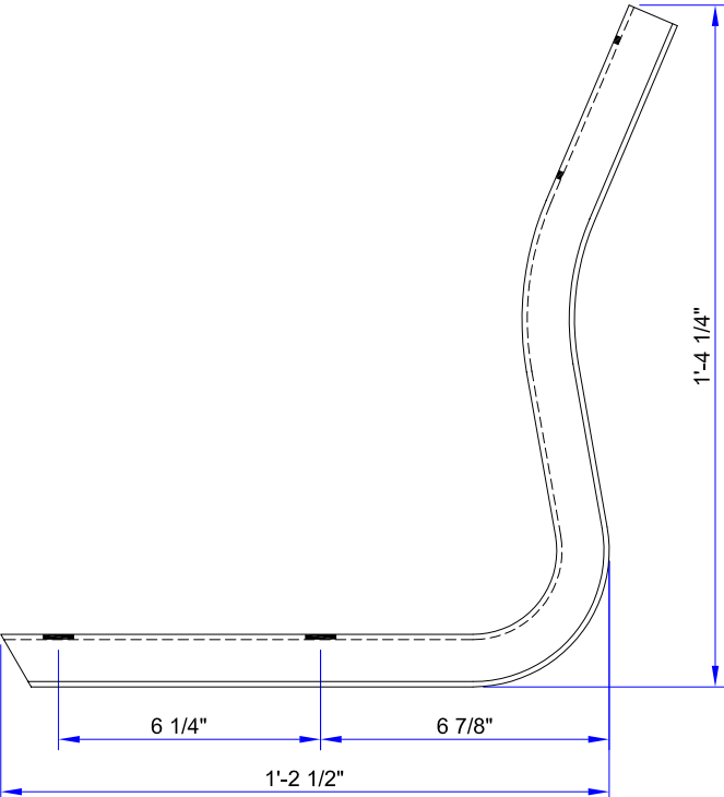
STANCHION ( ALCOA # T-3200 )
