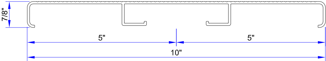
1 x 10 SC-RISER ( ALCOA # 70004 )
