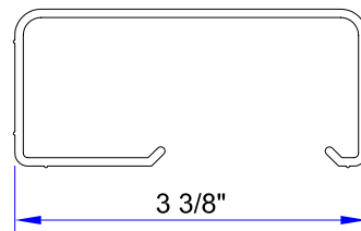
3 3/8" INSERT ( ALCOA # 67049 ) FOR 2 x 10 ( # 60772 )
