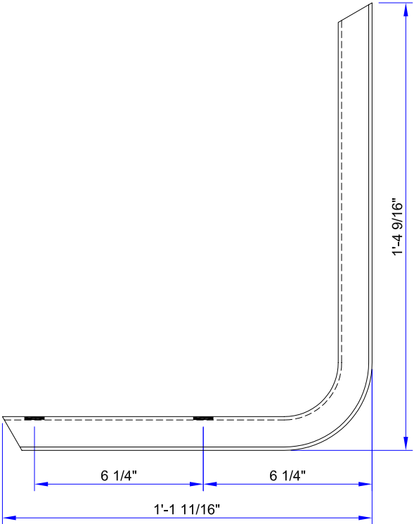
STANCHION ( ALCOA # T-5609 )
