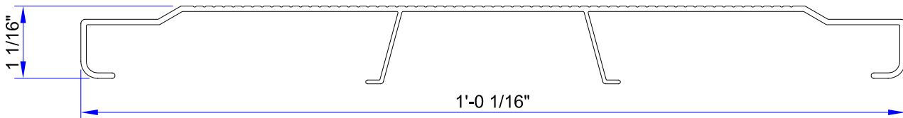
1 x 12 CI-RISER ( ALCOA # ????? )
