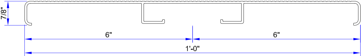
1 x 12 SC-RISER ( ALCOA # 70002 )
