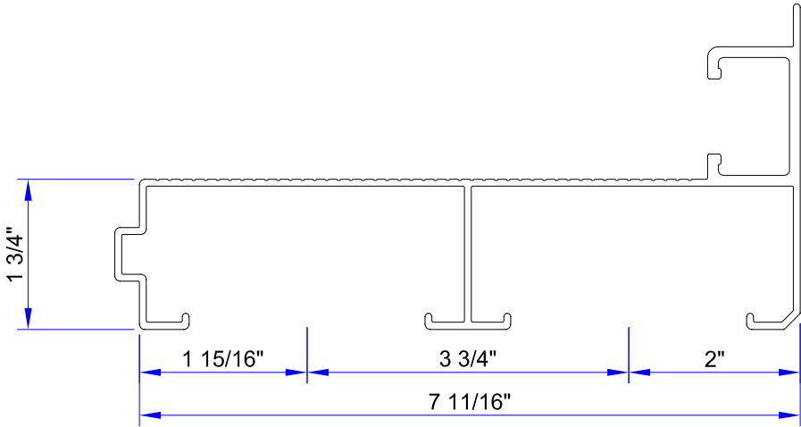
2 x 7 CI-HEEL ( ALCOA # 69800 )
