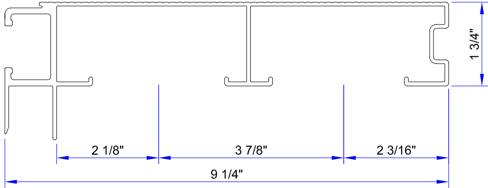
2 x 9 CI-NOSE ( ALCOA # 69804 )
