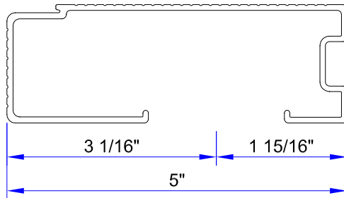
2 x 5 STEP NOSE ( ALCOA # 70014 )
