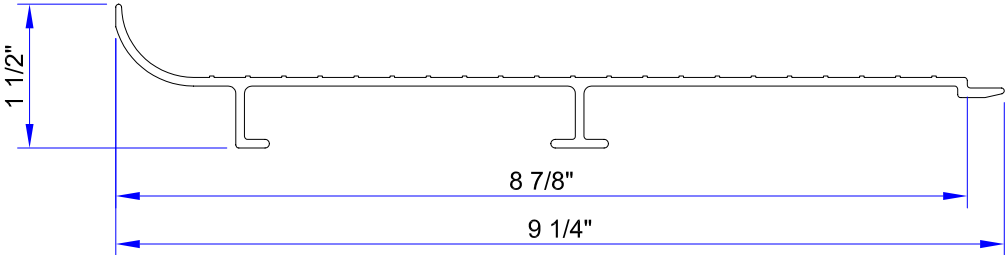
1 1/2 x 8 1/2 IL-RISER ( ALCOA # 69704 )
