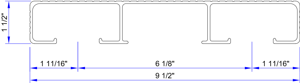
1 1/2 x 9 1/2 SEAT SUPPORT FOR PERMA CAP ( ALCOA# 67817 )
