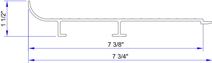
1 1/2 x 7 IL-RISER ( ALCOA # 68492 )
