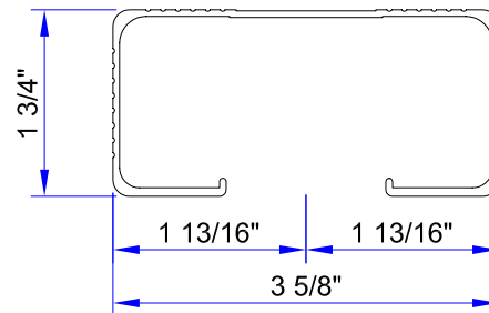
2 x 4 ( ALCOA # 14993 )
