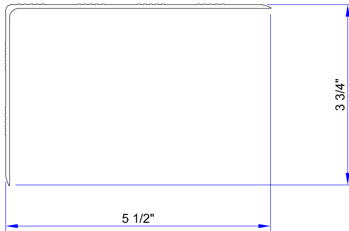
CLOSURE FOR SEMI-CLOSED DECK( ALCOA # 65987 )
