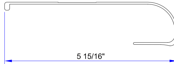
CONTOURED DISH BACK ( ALCOA # 11161 )
