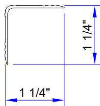
1 1/4" COLORED NOSE ( ALCOA # 68566 )
