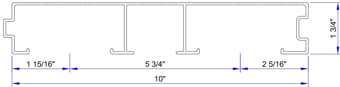
2 x 10 IL-DECK ( ALCOA # 69802 )
