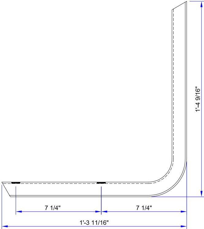
STANCHION ( ALCOA # T-294 )
