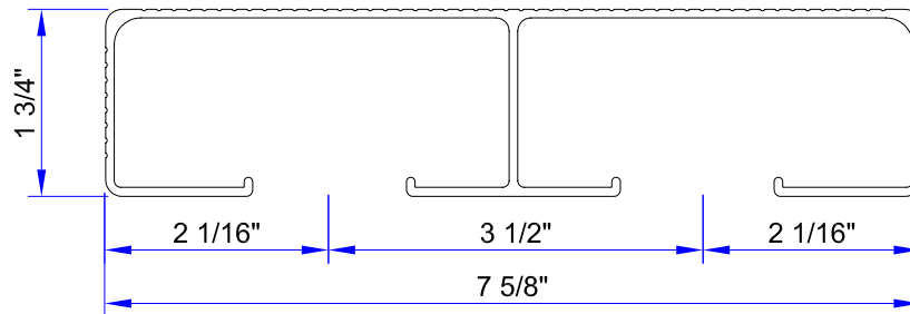
2 x 8 ( ALCOA # 65482 )
