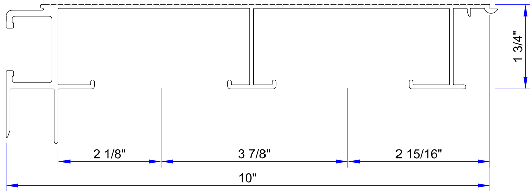
2 x 10 GI-NOSE ( ALCOA # 69942 )
