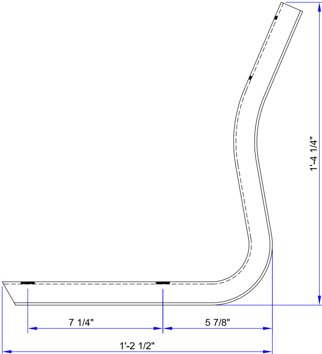
STANCHION ( ALCOA # T-2402 )
