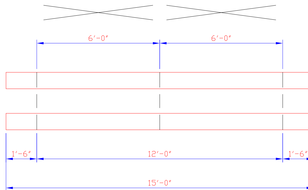
PLAN OF BLEACHER (1/4 SCALE)
