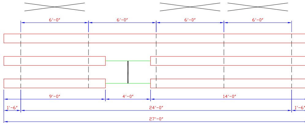
PLAN OF BLEACHER (1/4 SCALE)
