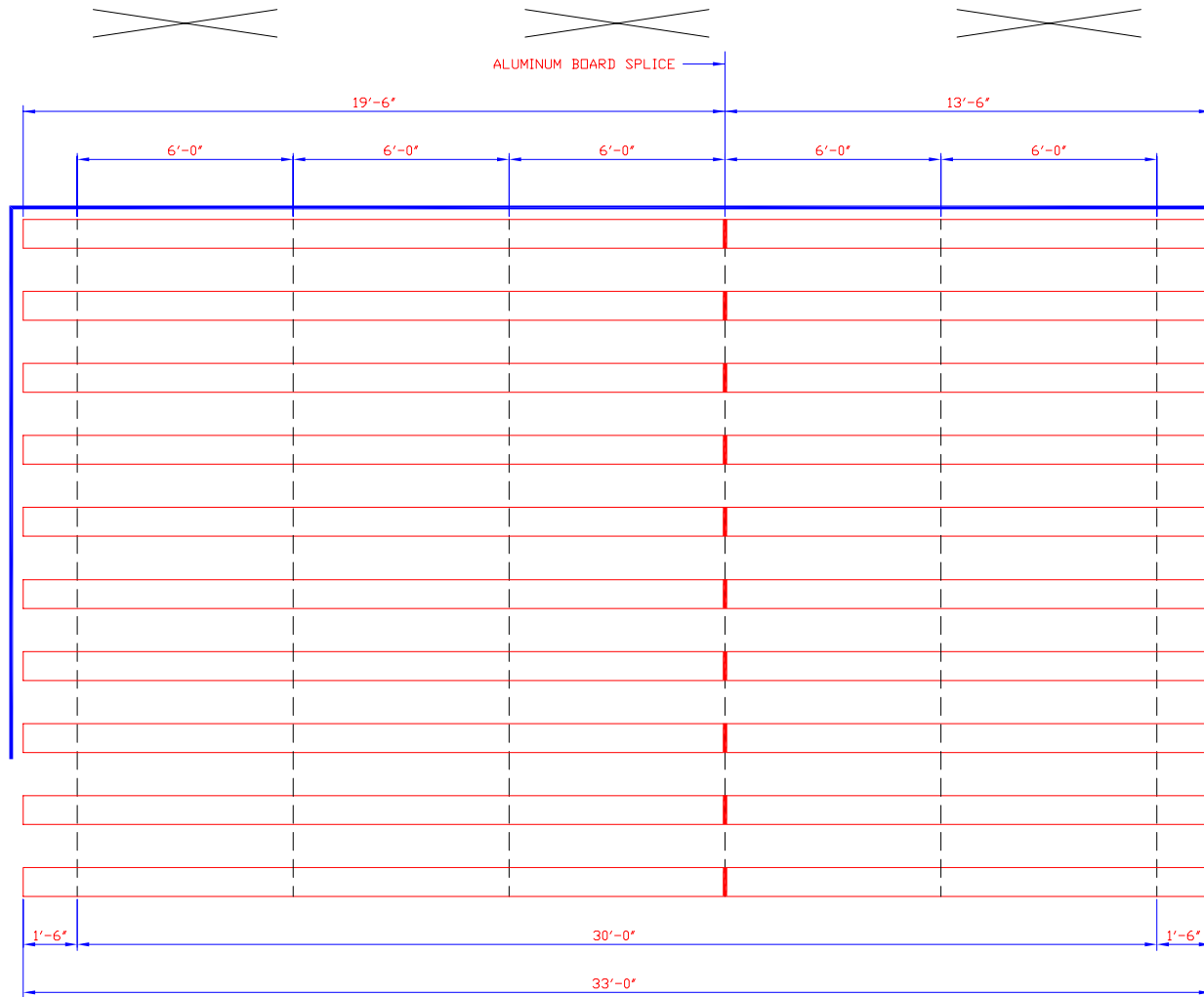
PLAN OF BLEACHER
