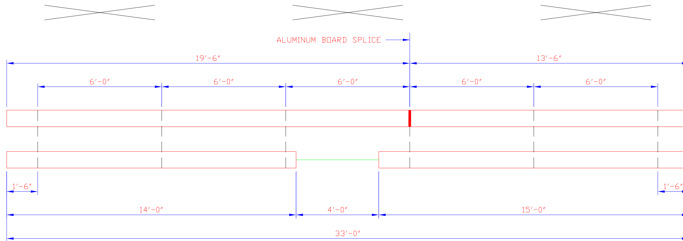
PLAN OF BLEACHER (1/4 SCALE)
