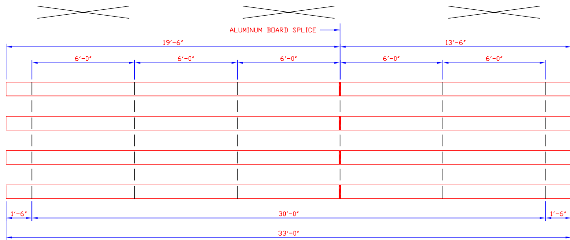
PLAN OF BLEACHER (1/4 SCALE)
